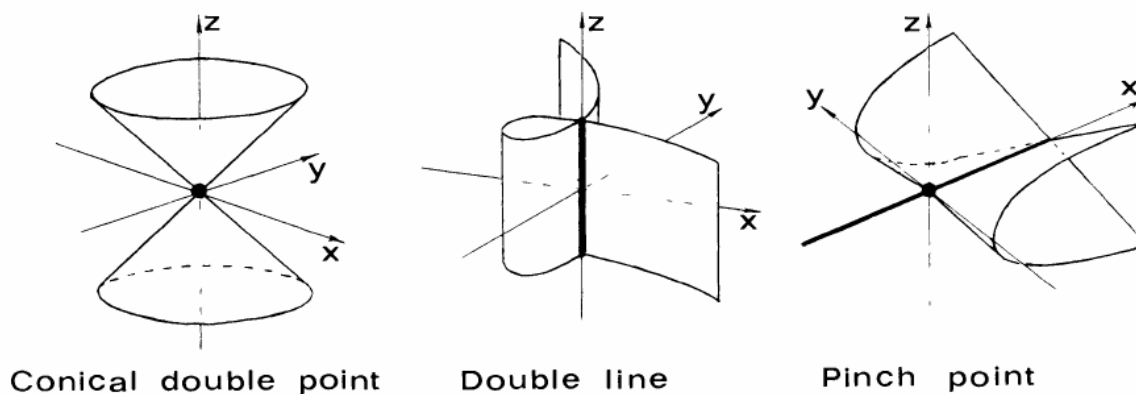
Figure 5. Surface singularities.
