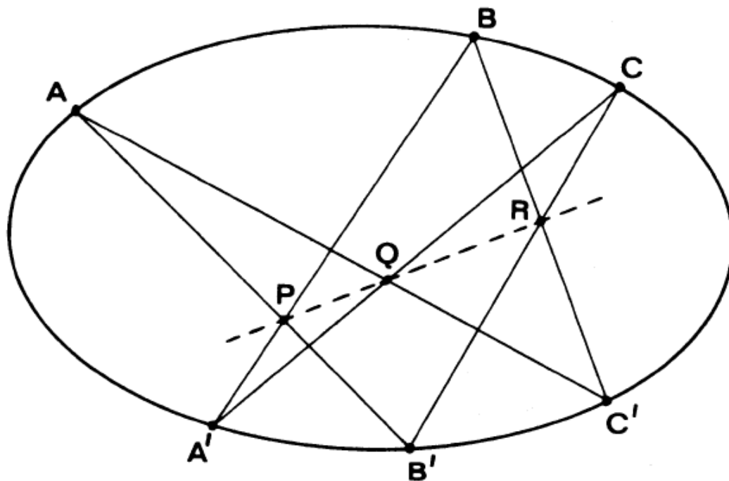
Figure 22. Pascal's theorem.
