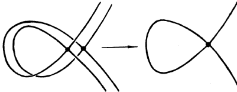
Figure 12. A finite étale covering.
