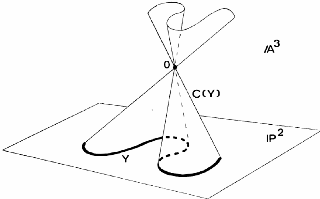
Figure 1. The cone over a curve in \mathbf{P}^2 .
