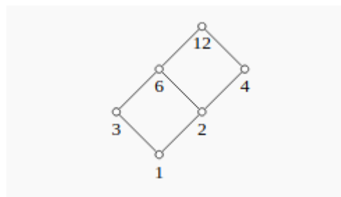
Figure 1: Divisibility Poset
