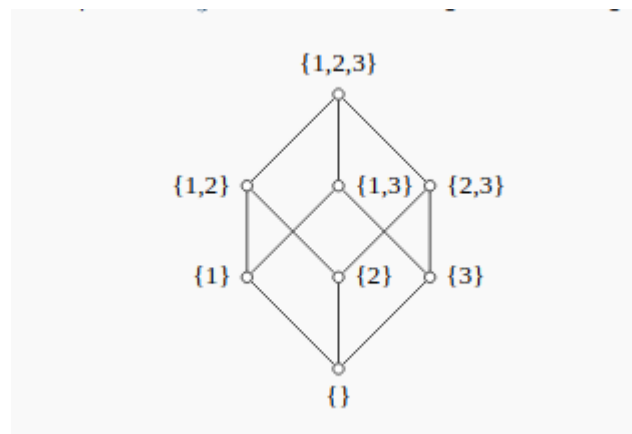
Figure 2: Subset Poset
