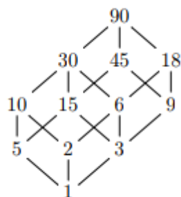
Figure 3: The Divisibility Poset on n = 90
