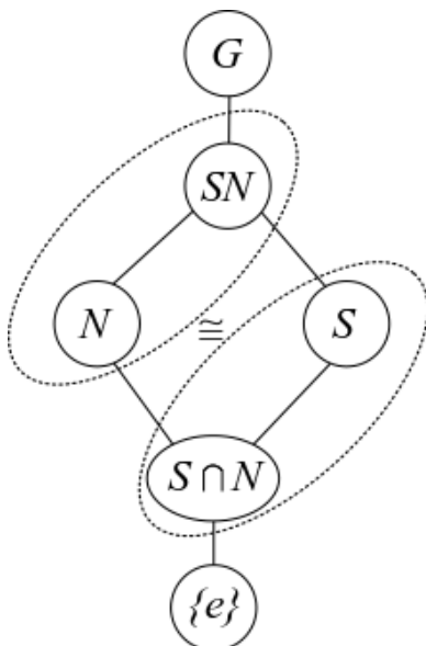
Figure 1: The 2nd “Diamond” Isomorphism Theorem
